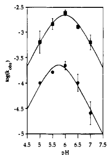
Figure 3. pH–rate profiles for 2 (2 mM)-promoted cleavage of (top) 2',3'-cAMP at 25 °C and (bottom) ApA (0.05 mM) at 50 °C.
