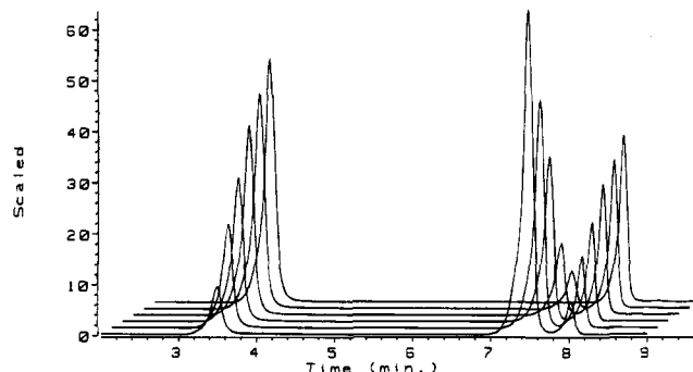
Figure 2. HPLC traces of 2 (2 mM)-promoted cleavage of 2',3'-cAMP at 25 °C, pH 6.0 (10 mM MES). Retention times are as follows: 3'-AMP = 3.5 min; 2',3'-cAMP = 7.5 min; 2'-AMP = 8 min. Reaction times are from foreground to background, 1, 3, 5, 10, 15, and 60 min.
