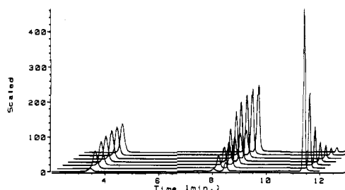
Figure 1. HPLC traces of 2 (2 mM)-promoted cleavage of ApA (0.05 mM) at 50 °C, pH 6.0 (10 mM MES). Retention times are as follows: 3'-AMP = 3.5 min; 2',3'-cAMP = 7.5 min; 2'-AMP = 8 min; adenosine = 8.5 min; ApA = 11.4 min. Reaction times are from foreground to background, 20, 100, 180, 260, 340, 420, and 500 min.
